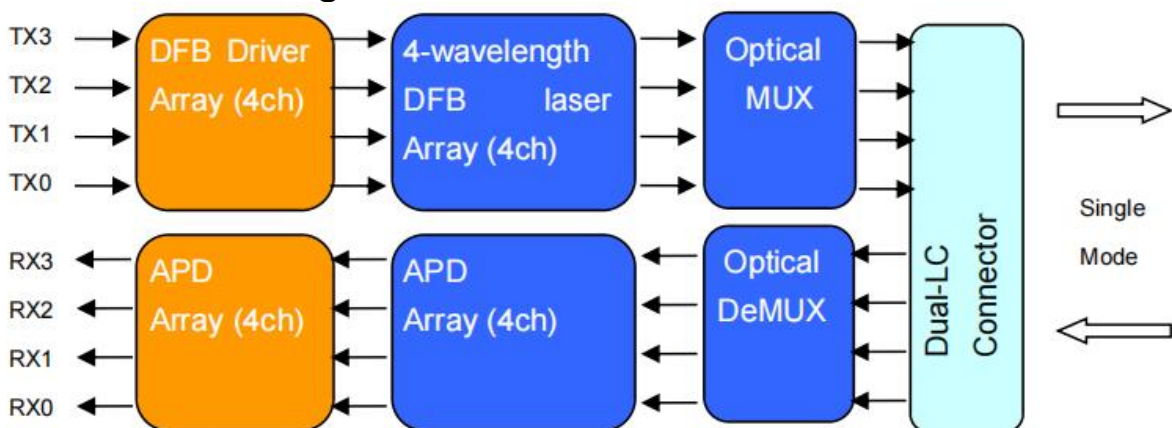
Figure 1: 40Gb/s QSFP ZR4 Transceiver Block Diagram
